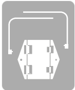
Wall mounting bracket with mounting kit with two plastic mounting ties
