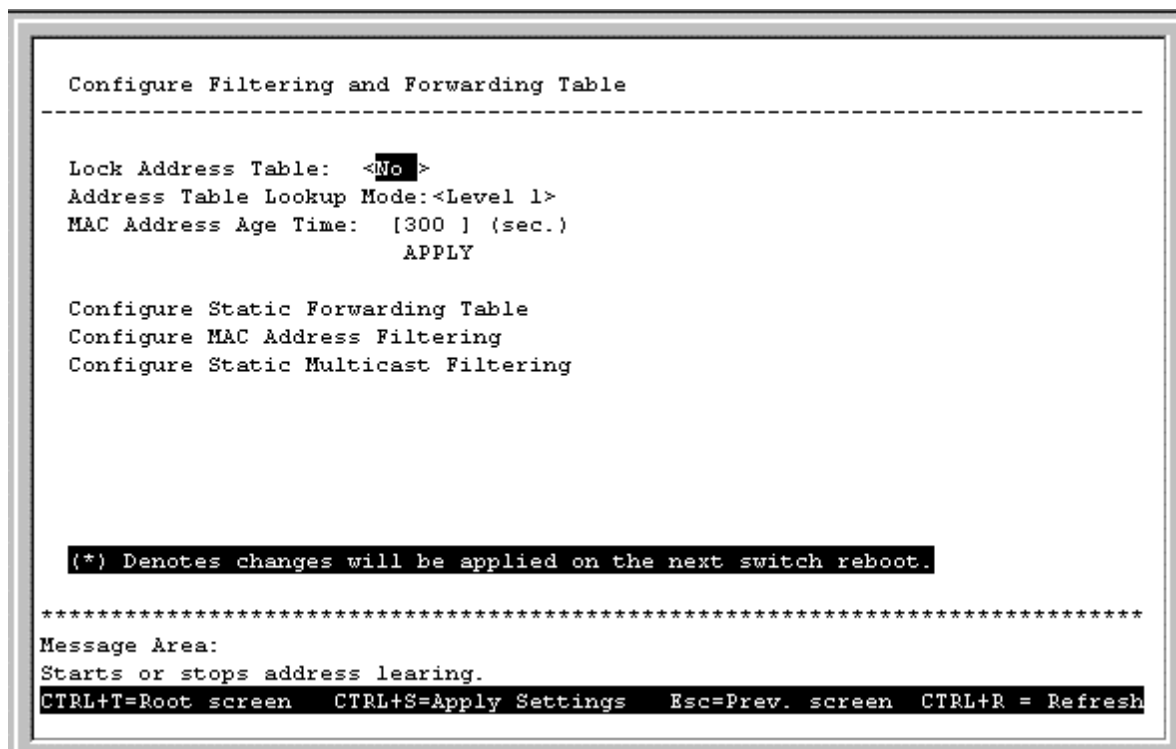
Figure 6-20. Configure Filtering and Forwarding Table screen
