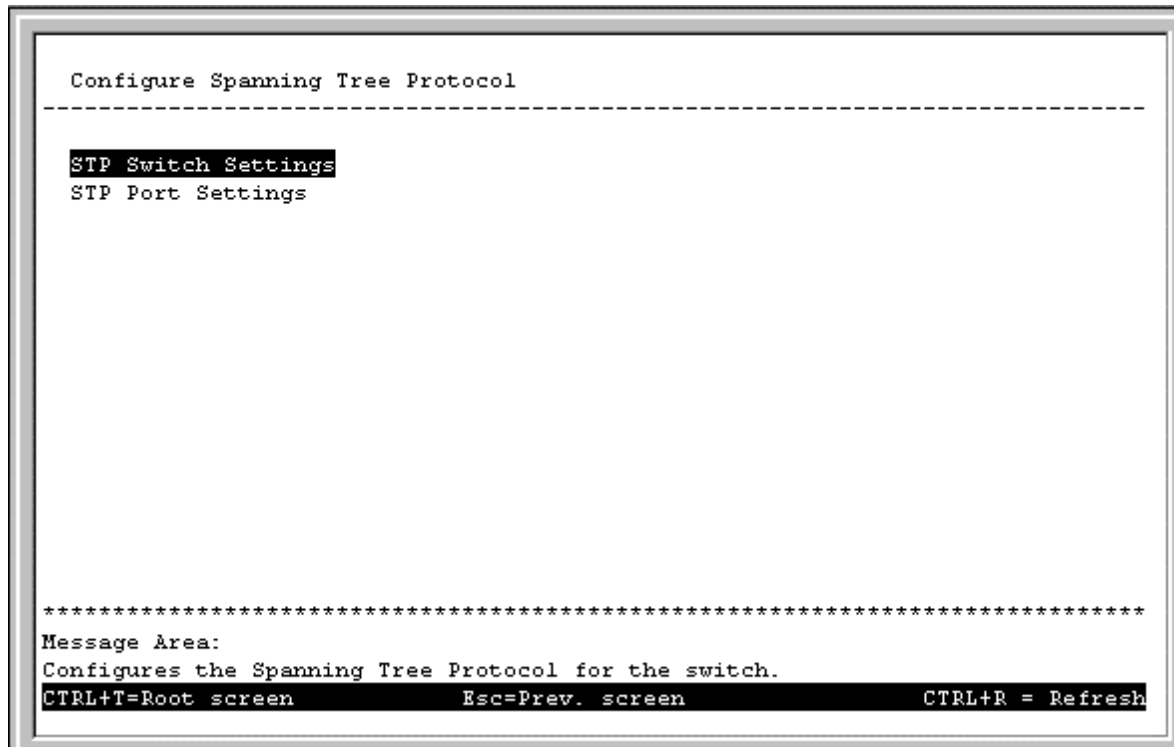
Figure 6-17. Configure Spanning Tree Protocol menu
