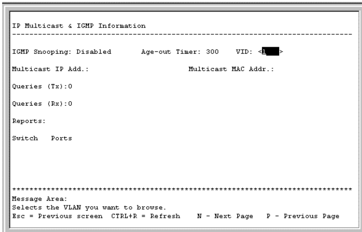
Figure 6-60. IP Multicast & IGMP Information screen
