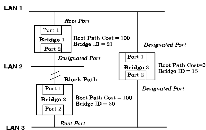
Figure 5-2. After Applying the STA Rules
