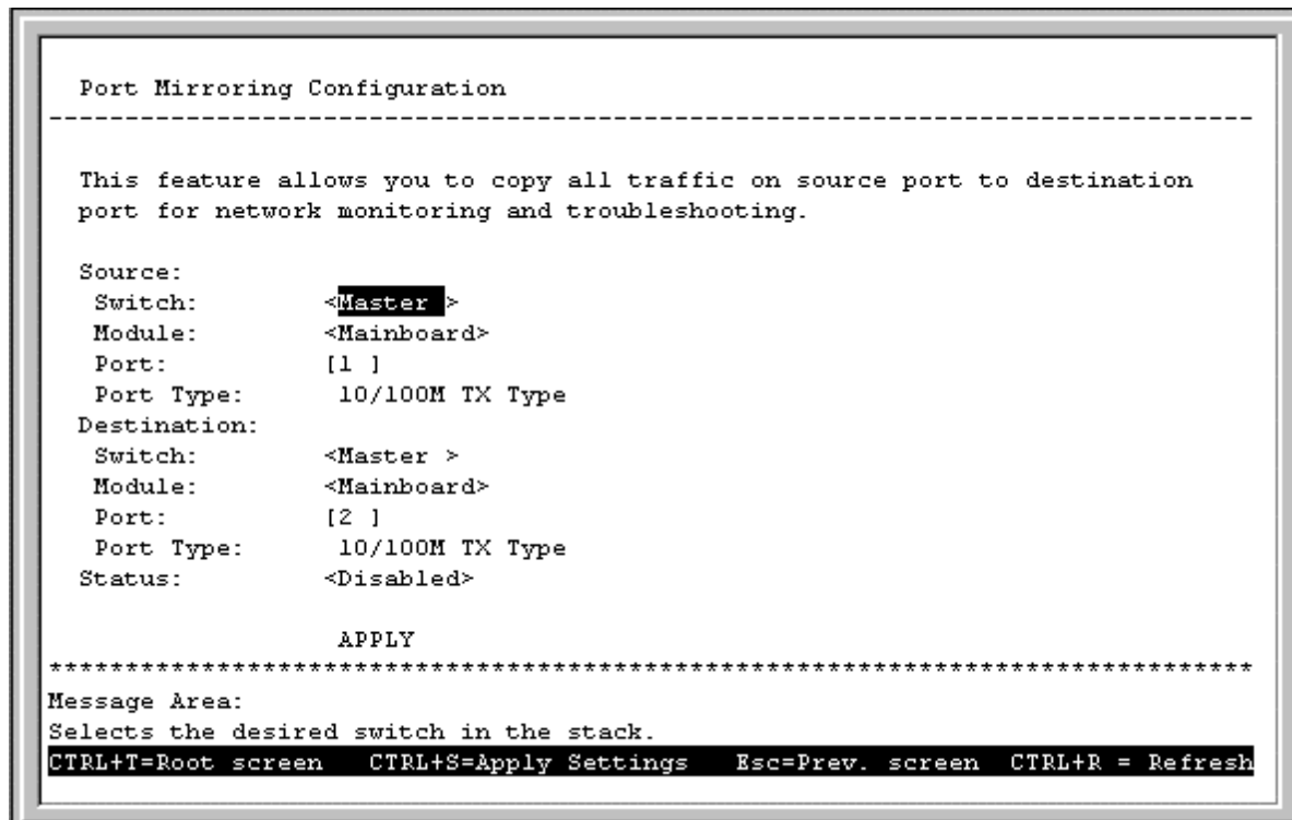
Figure 6-16. Port Mirroring Configuration screen
