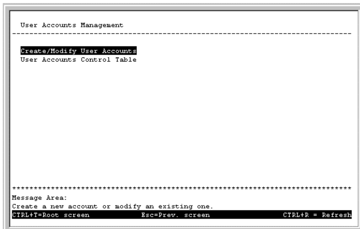
Figure 6-5. User Accounts Management menu
