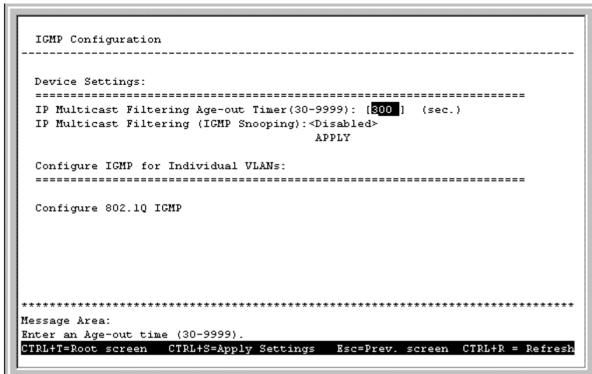
Figure 6-24. IGMP Configuration screen
