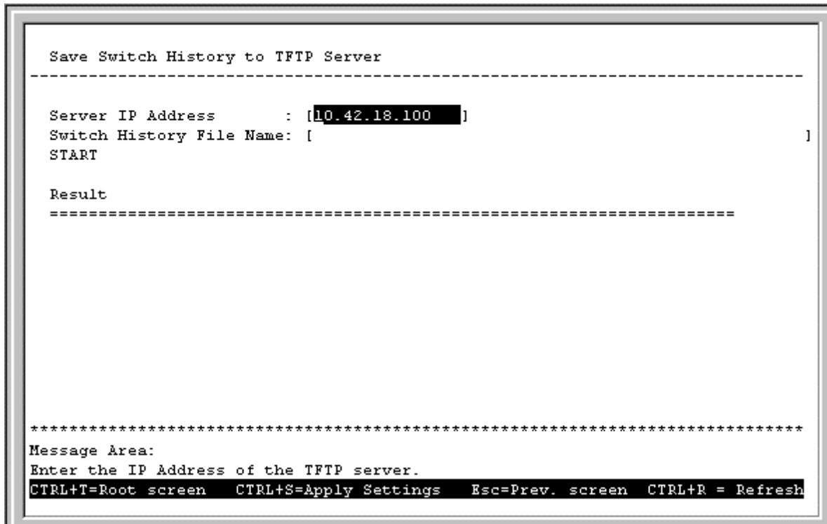
Figure 6-50. Save Switch History to TFTP Server screen
