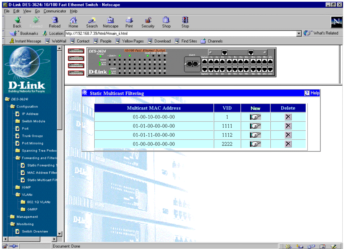
Figure 7-15. Static Multicast Filtering window
