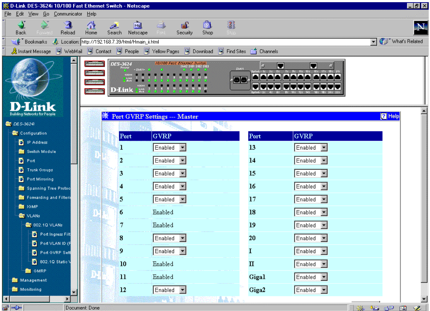
Figure 7-31. Port GVRP Settings window
