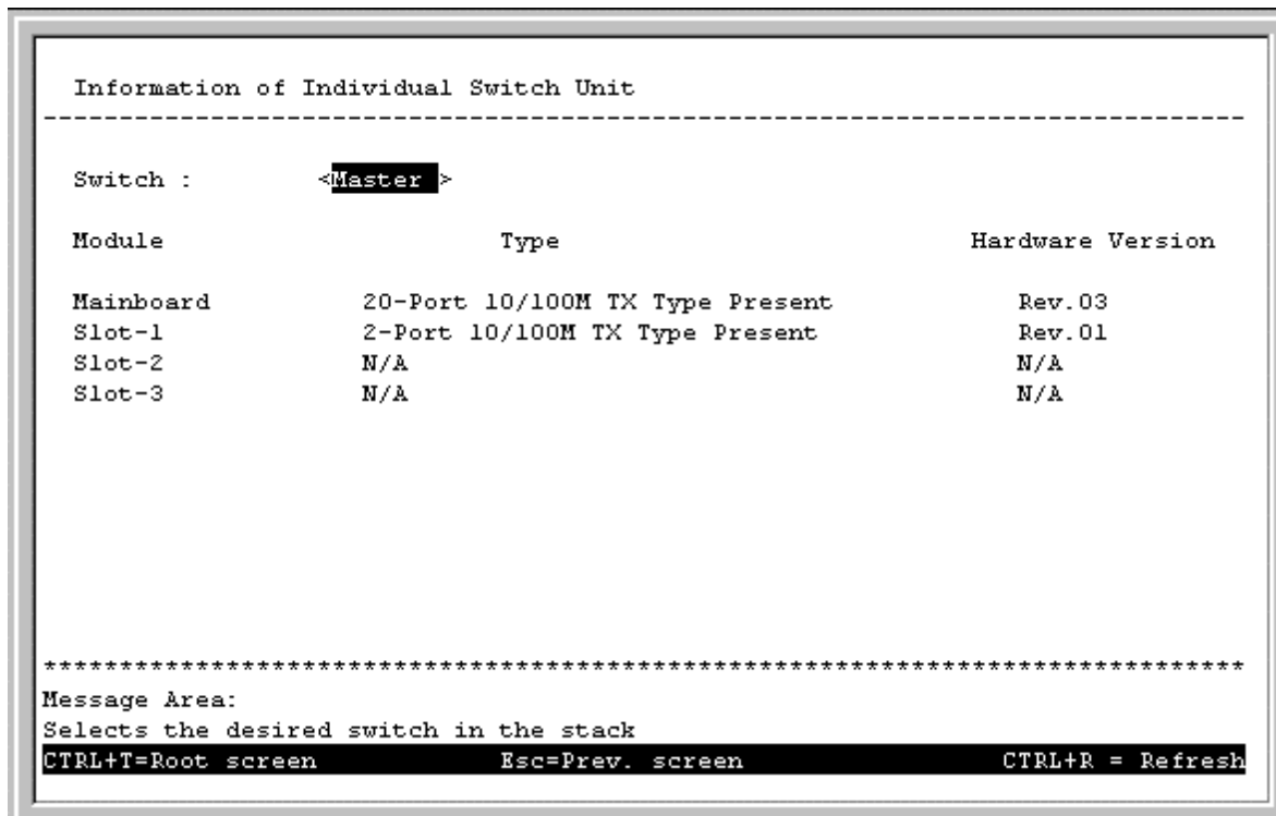
Figure 6-12. Information of Individual Switch Unit screen
