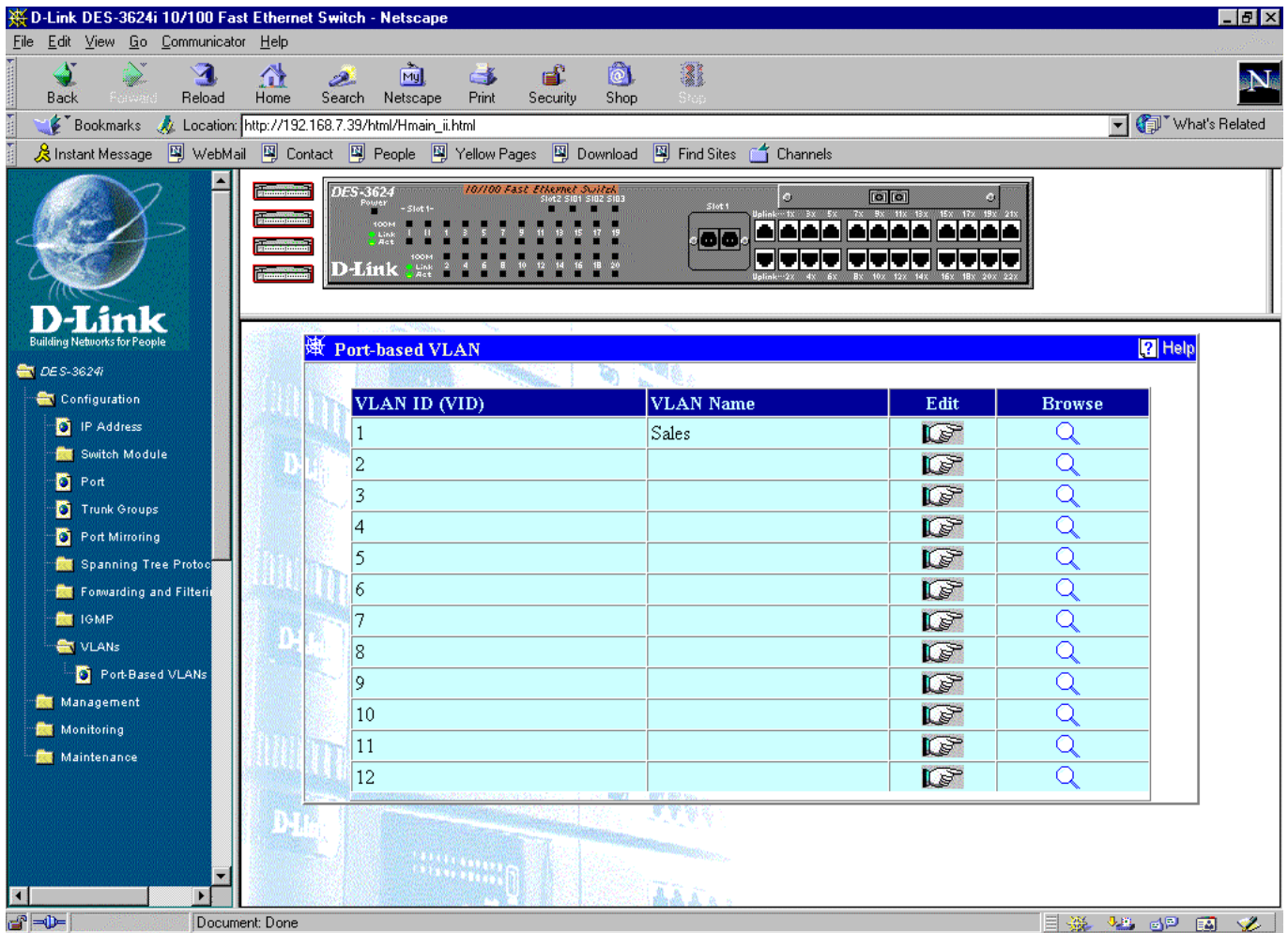
Figure 7-27. Port-based VLAN window
