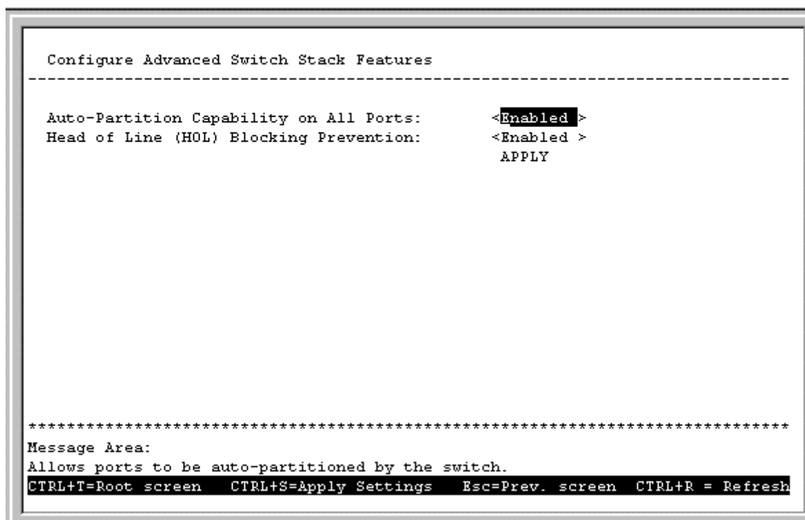
Figure 6-13. Configure Advanced Switch Stack Features screen
