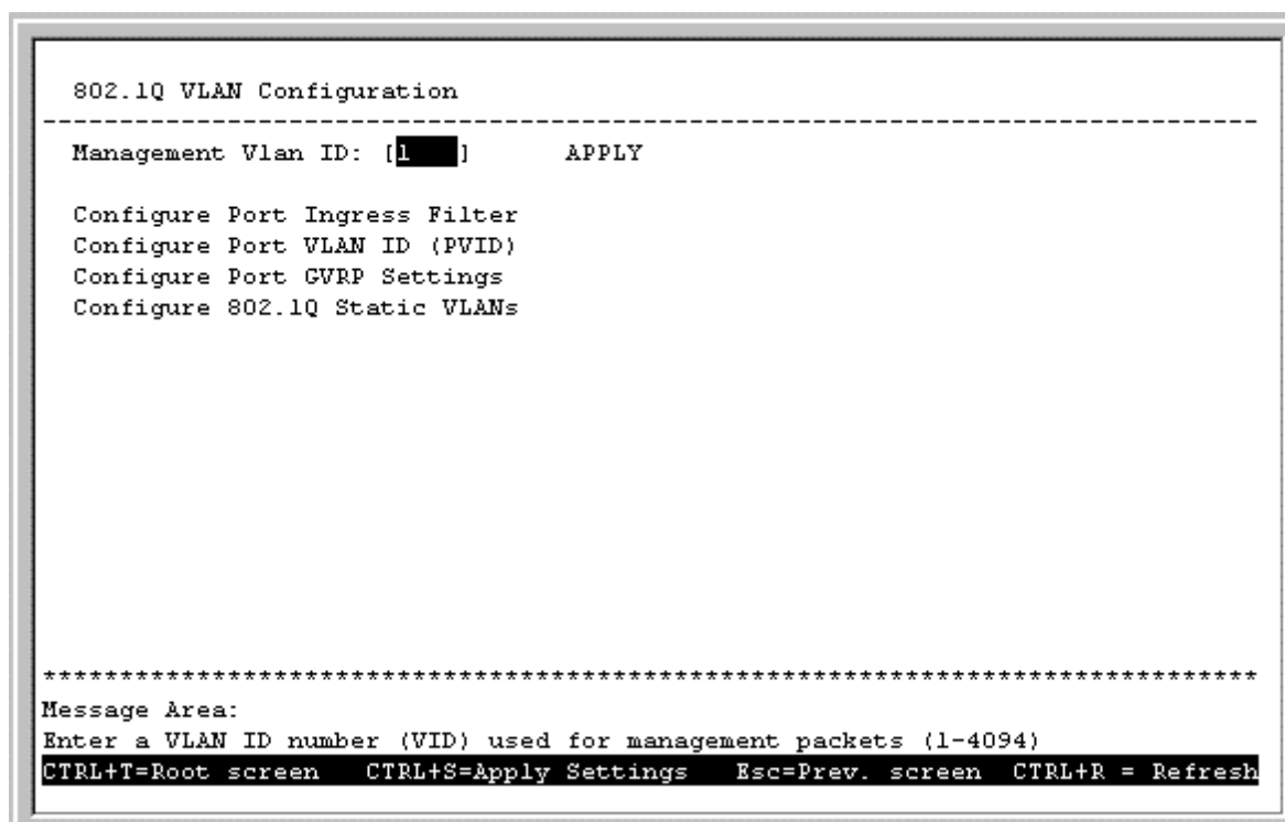
Figure 6-36. 802.1Q VLAN Configuration menu
