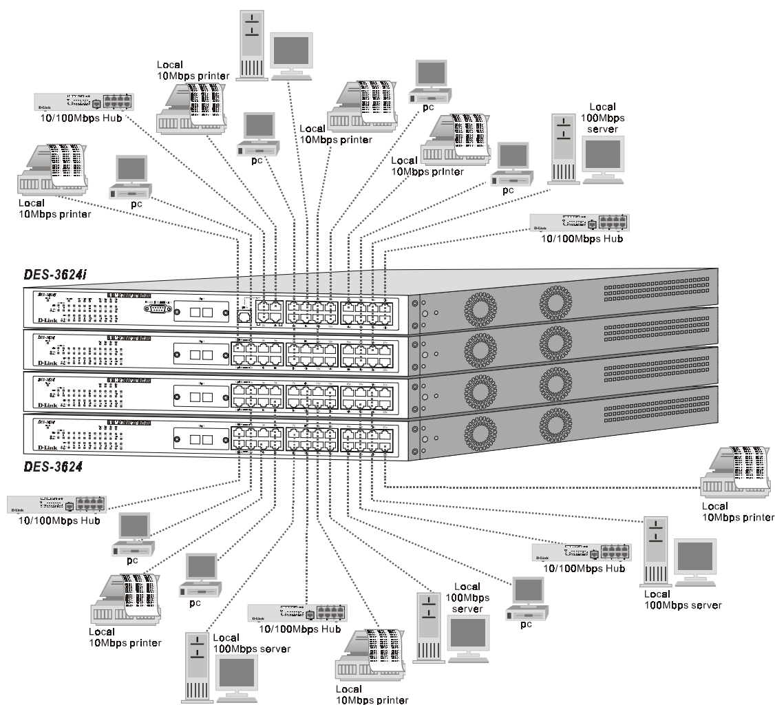
Figure 3-5. Switch stack with example of possible connections
