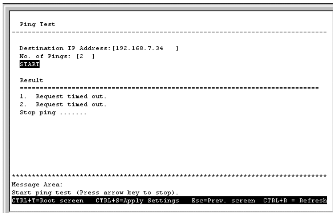
Figure 6-48. Ping Test screen
