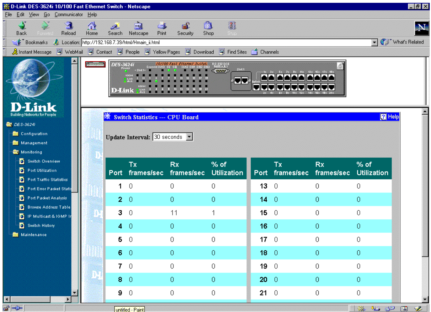
Figure 7-42. Switch Statistics window
