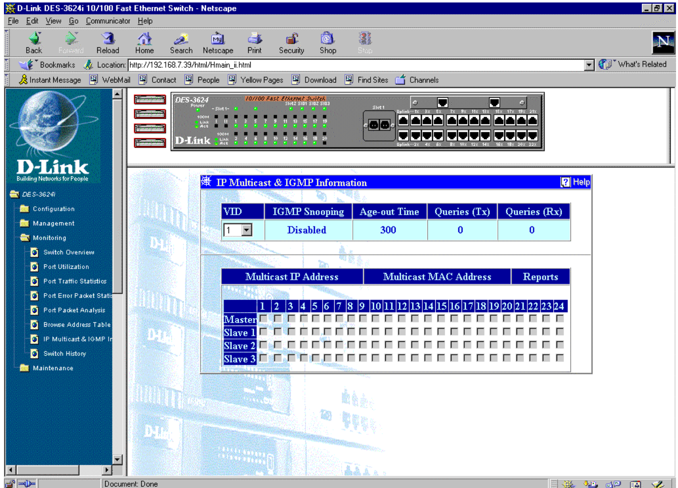
Figure 7-48. IP Multicast & IGMP Information window
