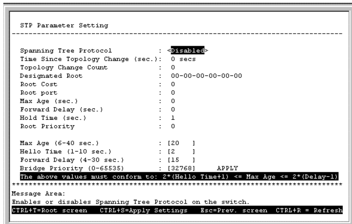
Figure 6-18. STP Parameter Setting screen
