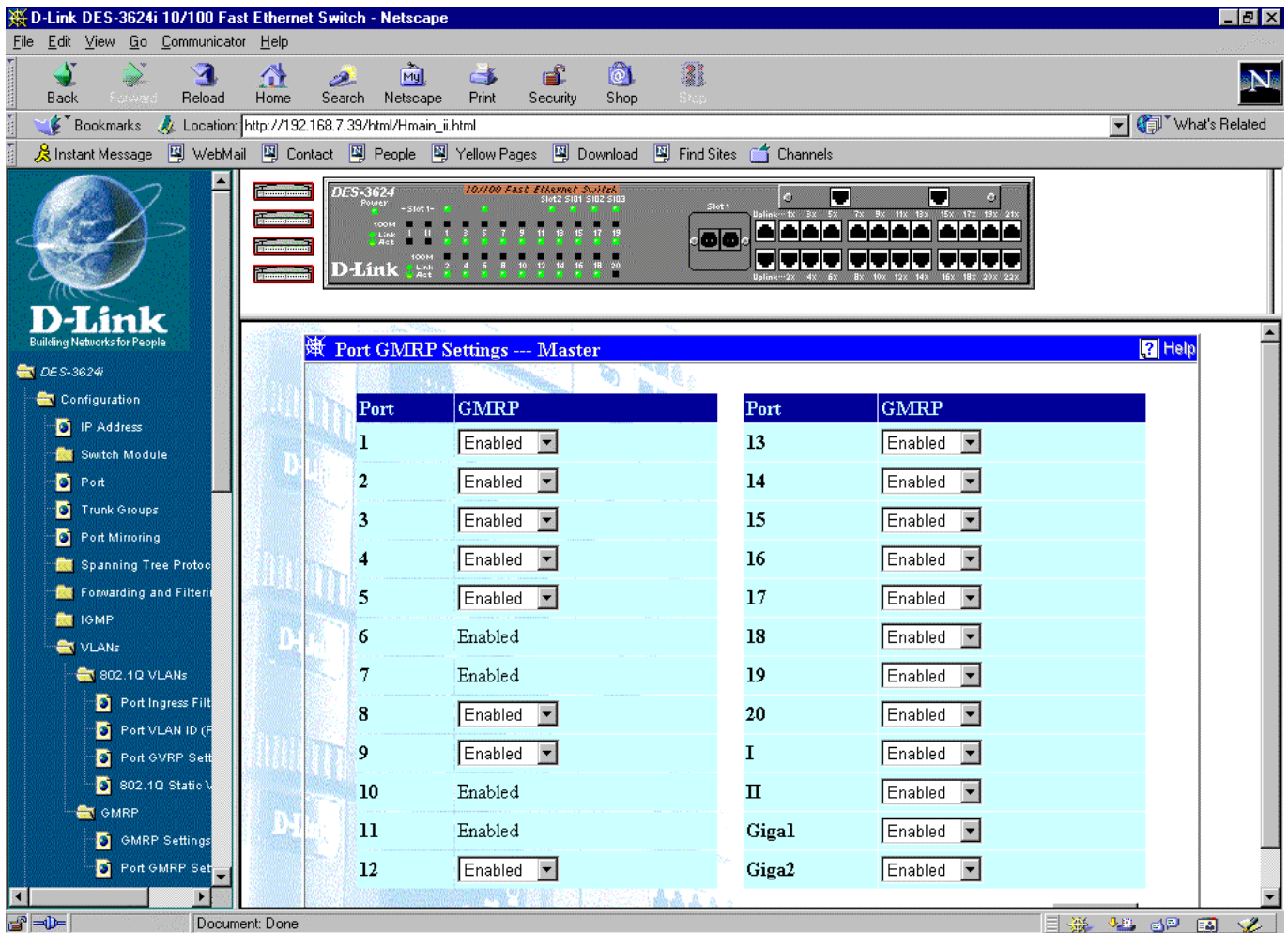
Figure 7-35. Port GMRP Settings window
