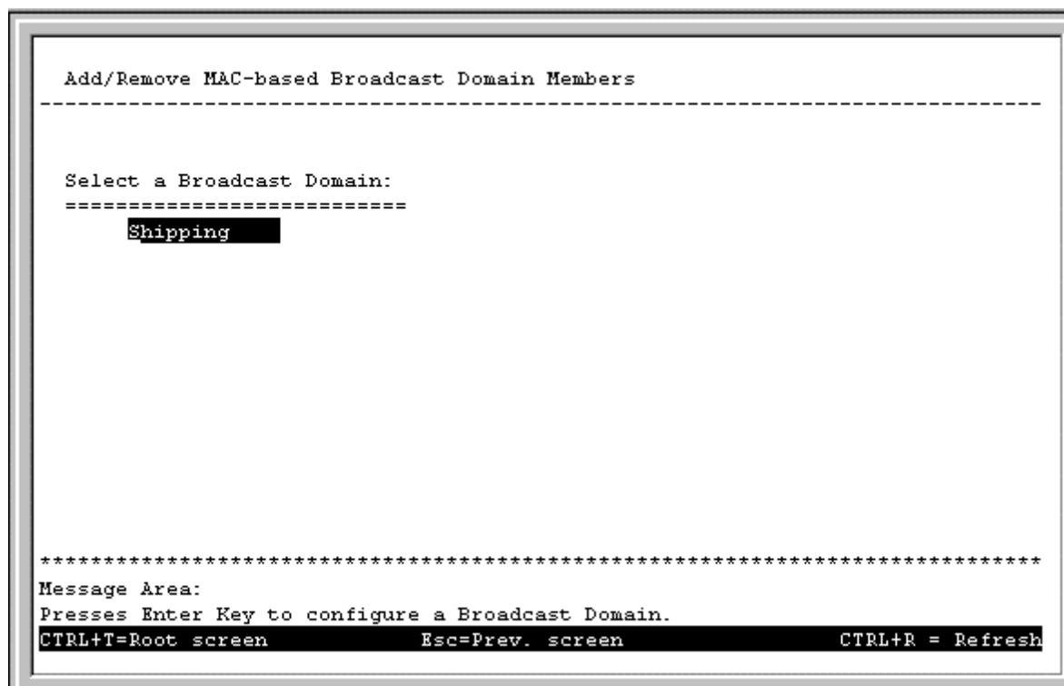
Figure 6-31. Add/Remove MAC-based Broadcast Domain Members screen
