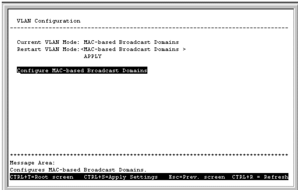
Figure 6-28. VLAN Configuration screen
