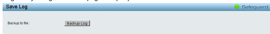
Figure 5.7 – Save Log
