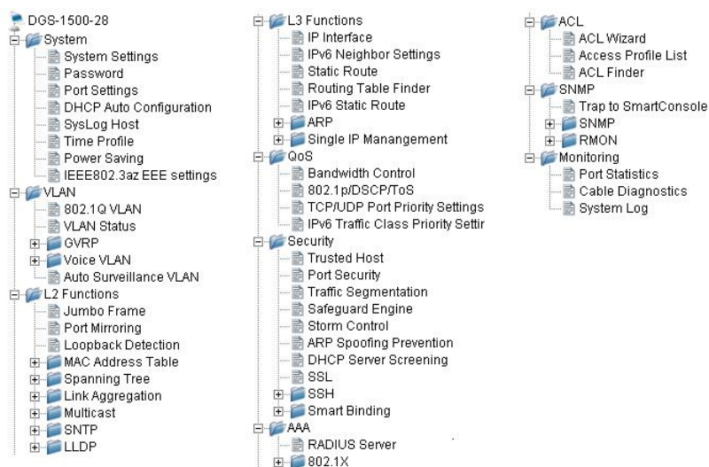
Figure 5.16 –Function Tree
