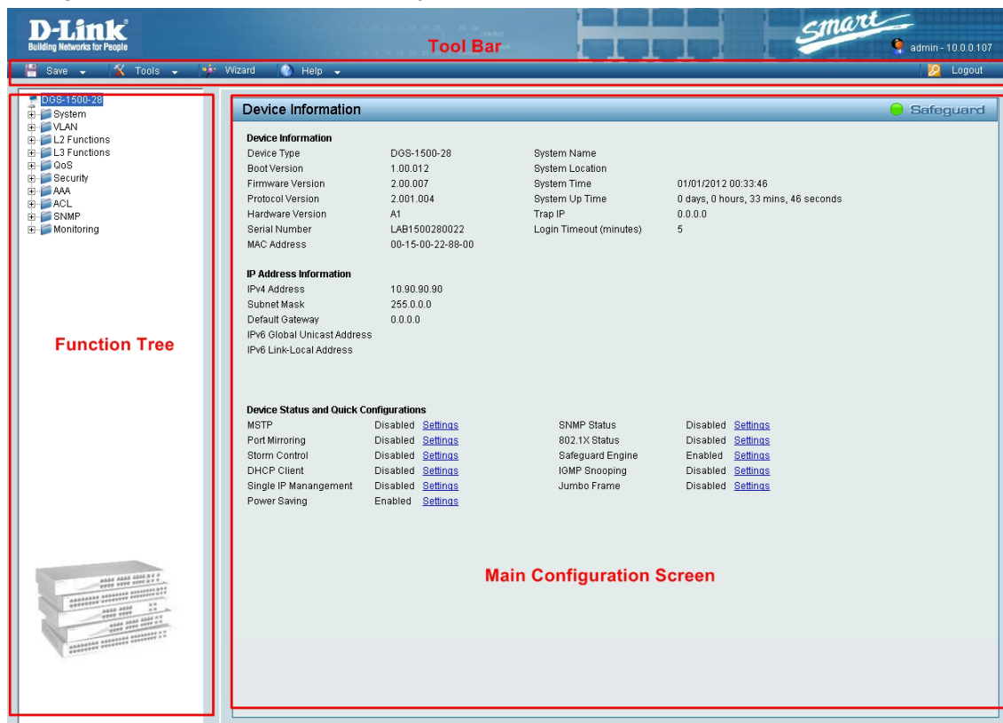
Figure 5.4 – Web-based Management
