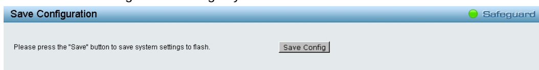
Figure 5.6 – Save Configuration
