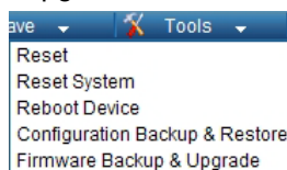
Figure 5.8 – Tool Menu
