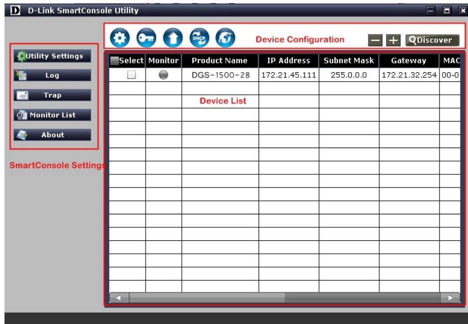
Figure 4.1 – SmartConsole Utility
