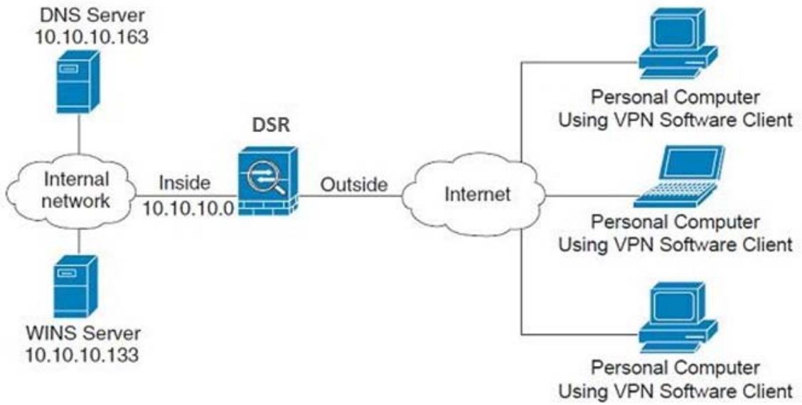
Figure 76: Example of three IPsec client connections to the internal network through the DSR IPsec gateway
