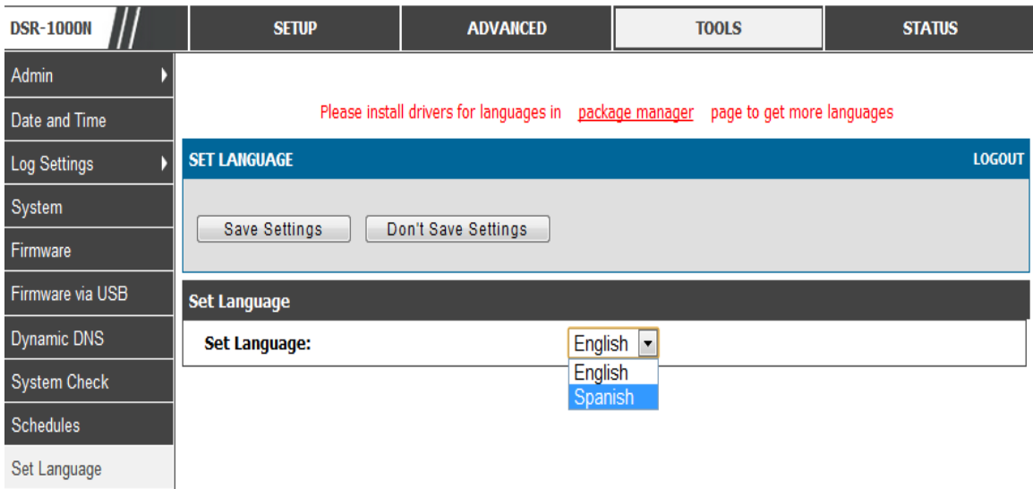
Figure 140: Localization
