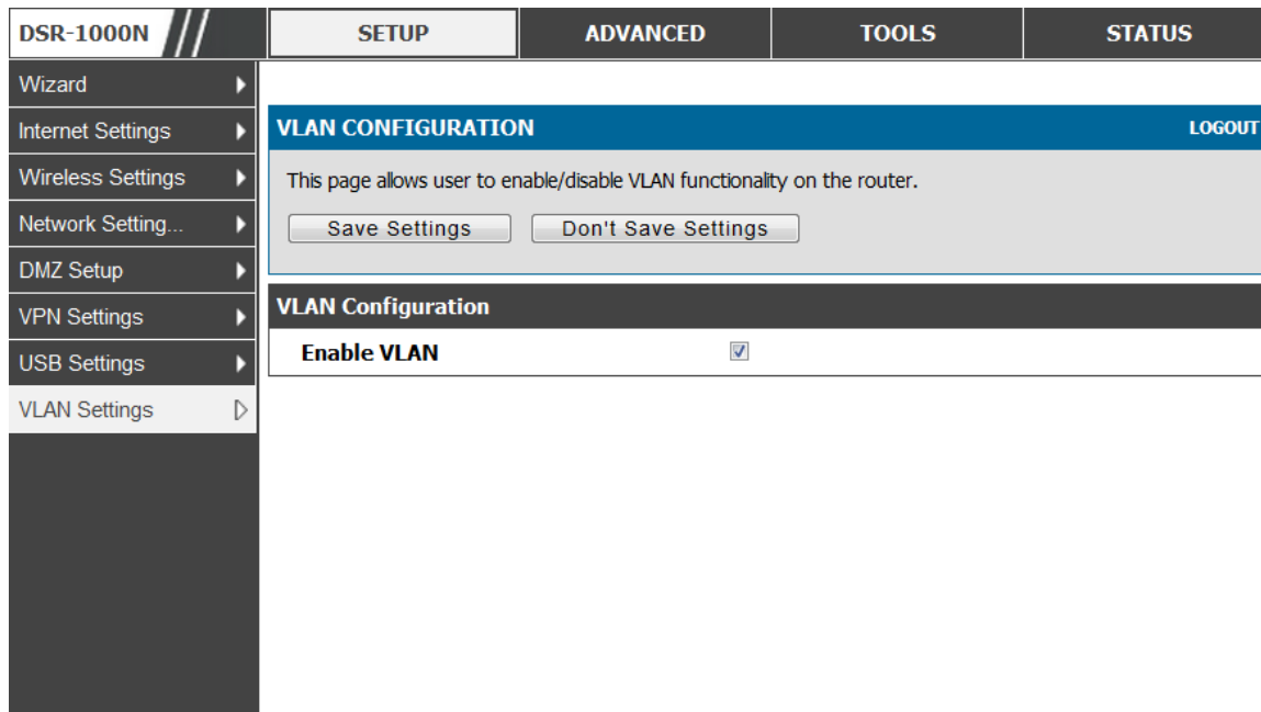
Figure 11: VLAN Configuration
