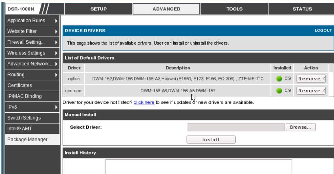
Figure 119: Device Drivers
