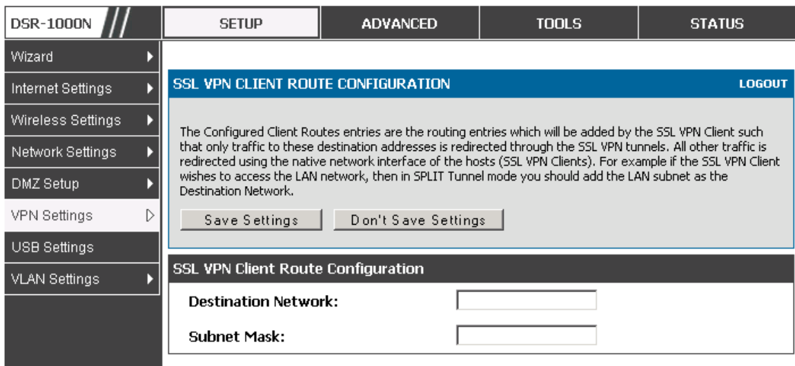
Figure 104: Configured client routes only apply in split tunnel mode
