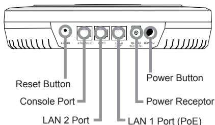
Figure 2. DWL-8620AP Rear Panel
