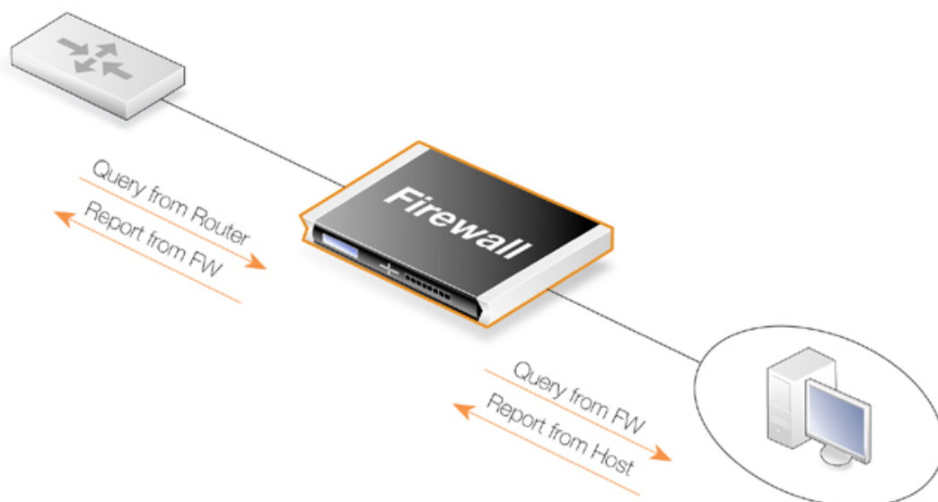
Figure 4.17. Multicast Proxy Mode
