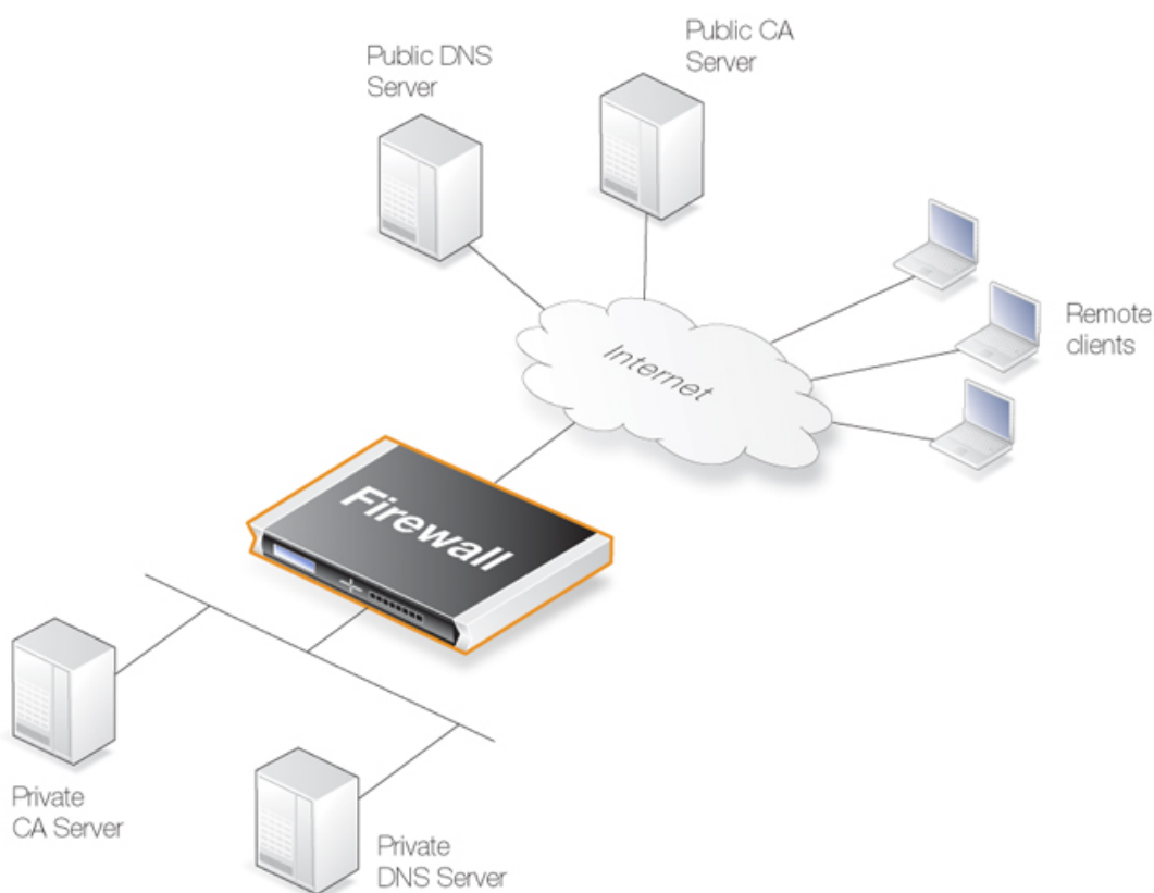
Figure 9.7. Certificate Validation Components
